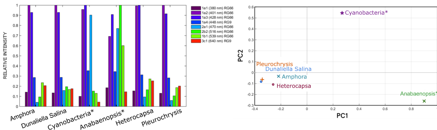
Relative pigment composition of different algae and cyanobacteria (marked with *) (left) and resulting score plot after analyzing the data by the means of the principal component analysis. Both cyanobacteria were separated clearly from the rest (right).
